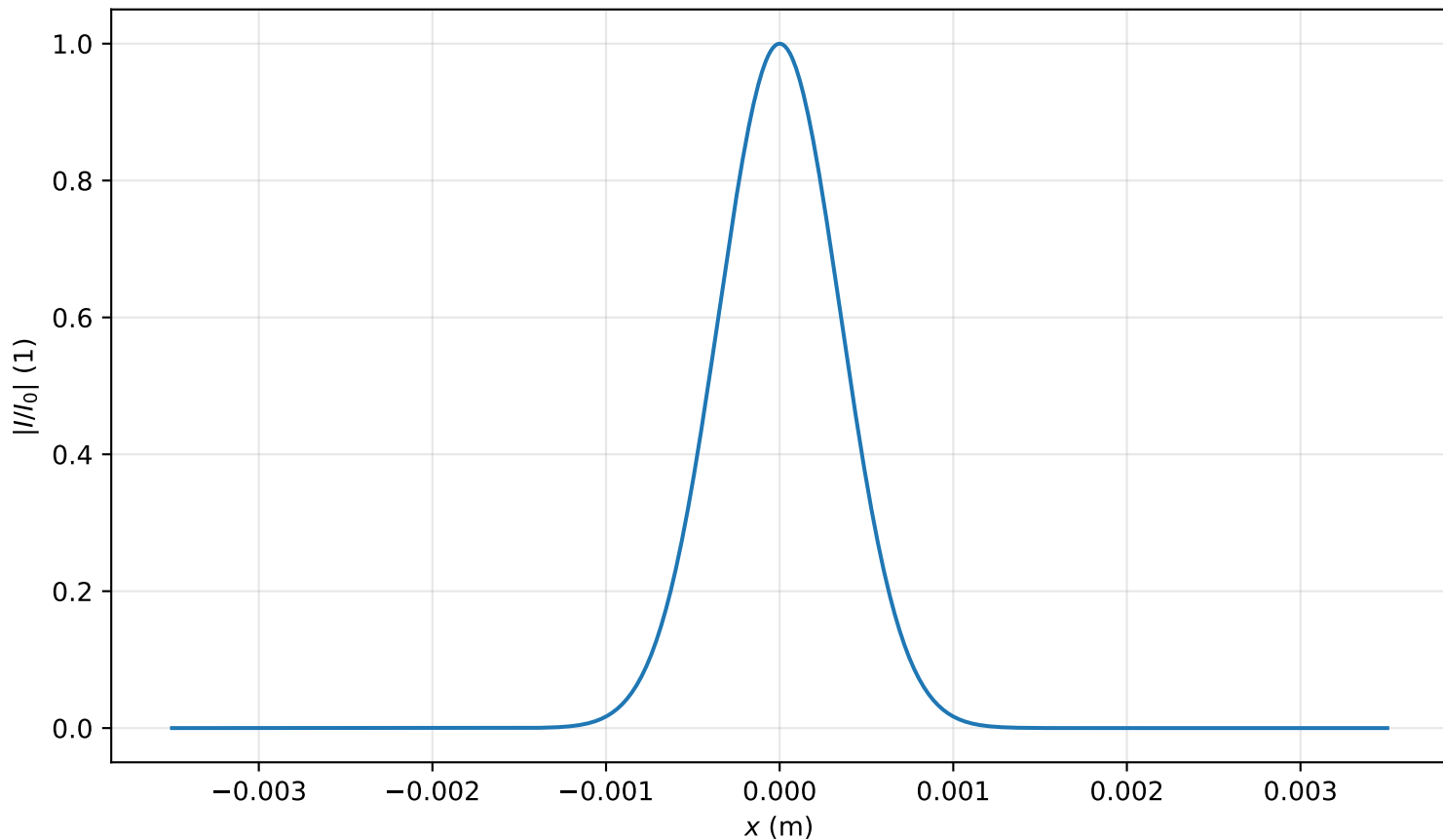
Intensity profile I(x, y = 0, z = 0.000m)/I_0 , P_{in}=0.6P_{cr} , artificial time
